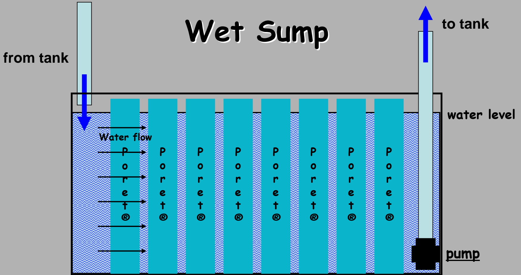
Side view wet sump
