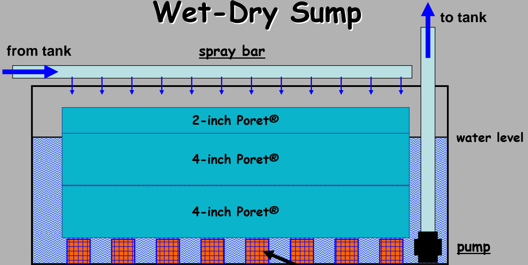
Side view wet-dry sump
